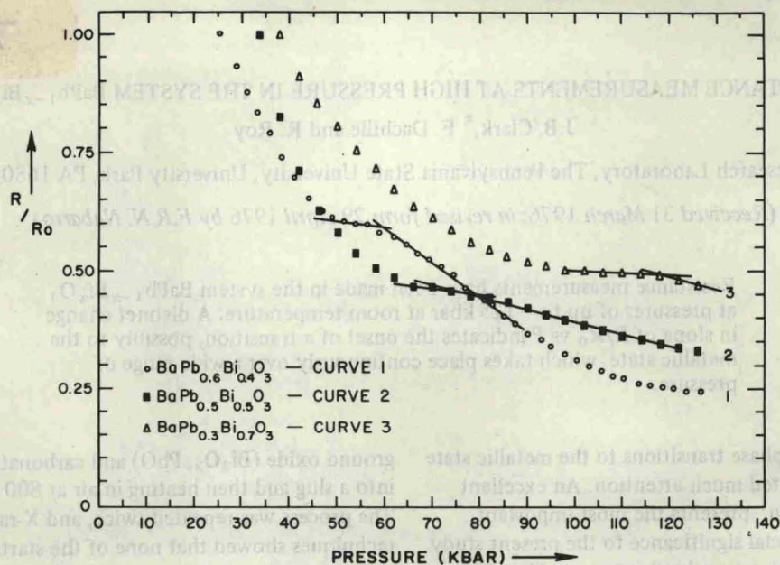
Fig. 2. Results obtained from 2-wire resistance measurements to \sim 125 kbar on: (1) \text{BaPb}_{0.6}\text{Bi}_{0.4}\text{O}_3 ; (2) \text{BaPb}_{0.5}\text{Bi}_{0.5}\text{O}_3 ; (3) \text{BaPb}_{0.3}\text{Bi}_{0.7}\text{O}_3 .
